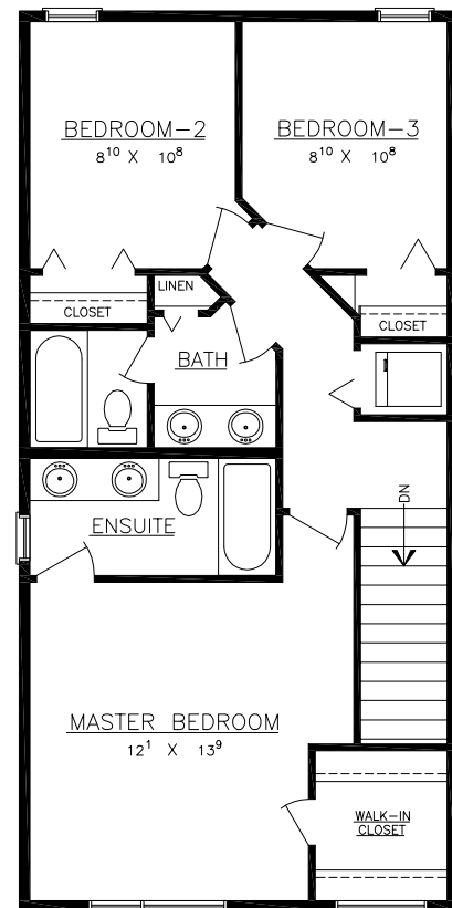
SECOND FLOOR AREA = 741 S.F.
